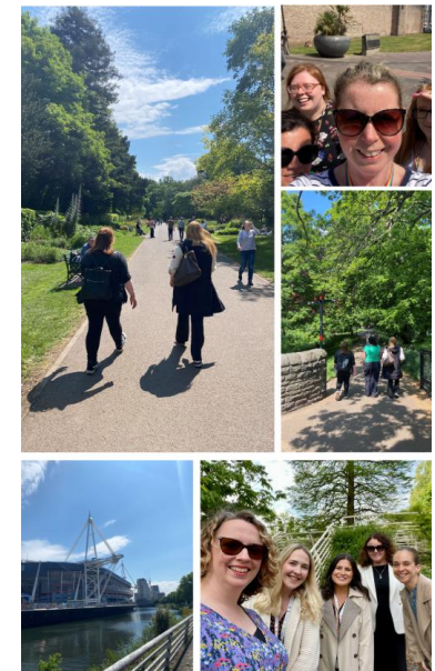
Cardiff (1,618,321 steps)
